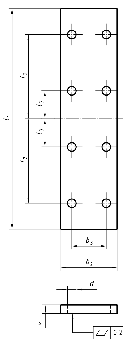
Figure 6 — Fishplate dimensions
