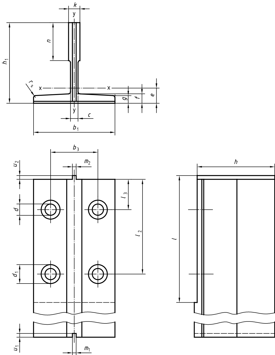
Figure 3 — Machined guide rail
